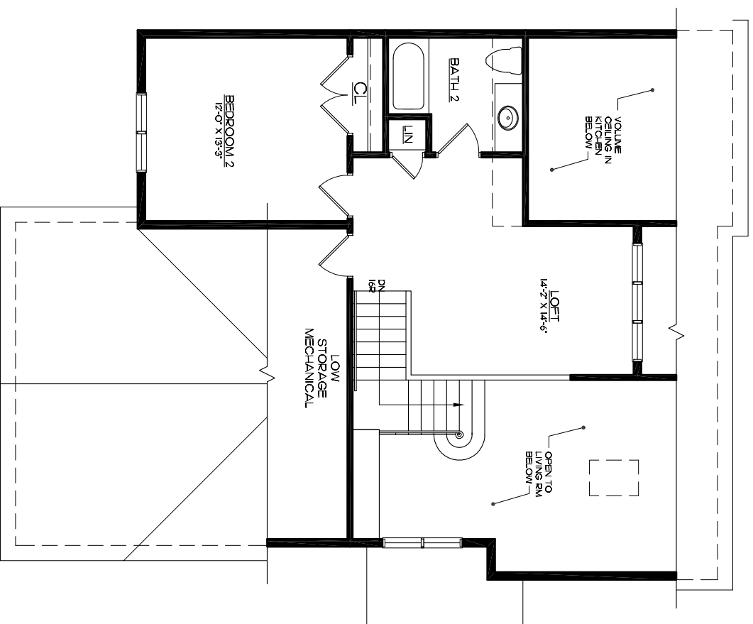
Second Floor Plan - Unit A Scale: 1/4" = 1'-0" 466 s.f.
