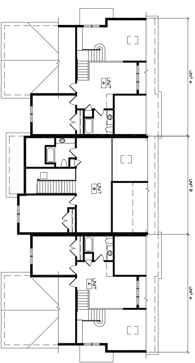
SECOND FLOOR PLAN - 3 UNIT BUILDING (BLDG. 3 & 5) Scale: 1/8" = 1'-0"
