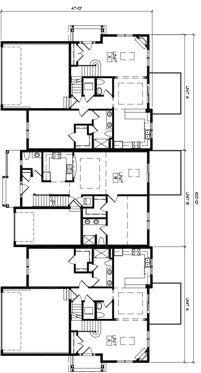
FIRST FLOOR PLAN - 3 UNIT BUILDING (BLDG. 3 & 5) Scale: 1/8" = 1'-0"
