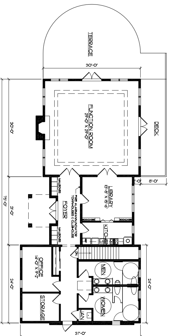
FIRST FLOOR PLAN - CLUBHOUSE (BLDG. 6) Scale: 1/8" = 1'-0" (2346 S.F.)
